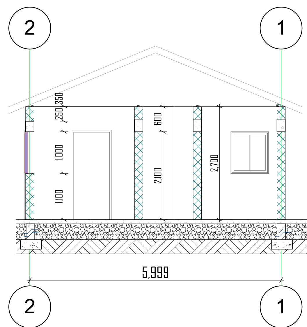
Section
