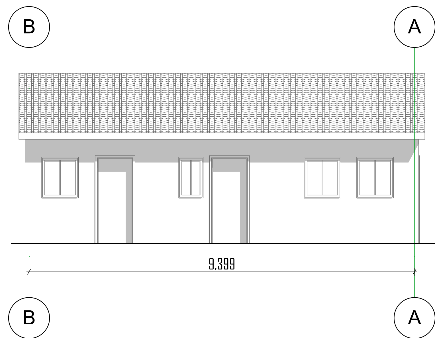
Elevation-01
