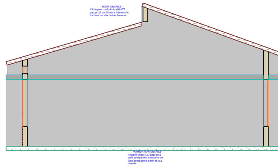
SECTION A
