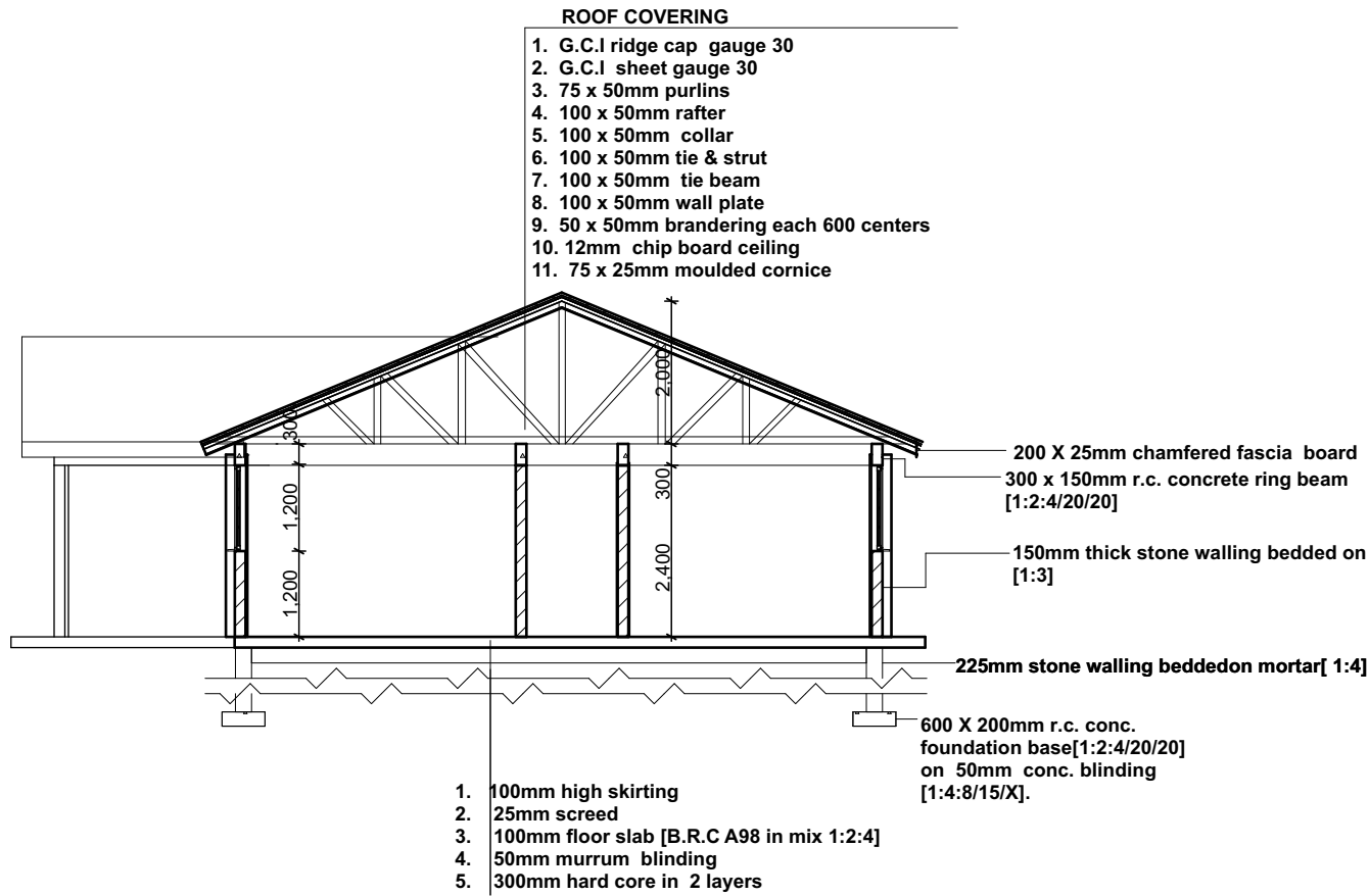
SECTION X-X
