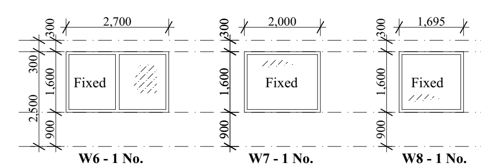
WINDOW SCHEDULE
