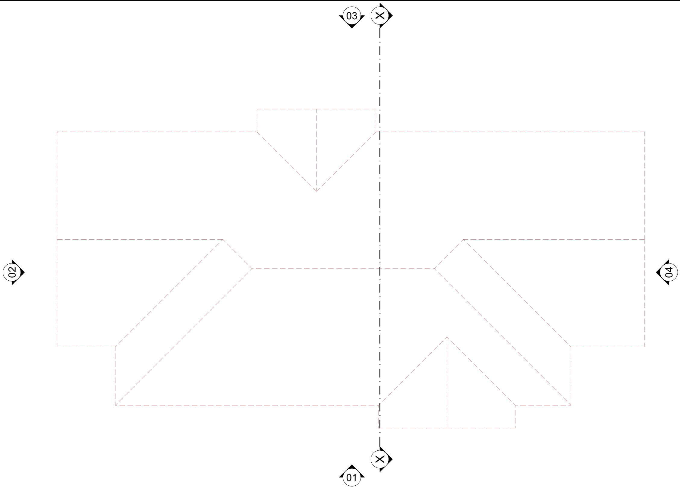
ROOF PLAN LAYOUT - SCALE 1:100
