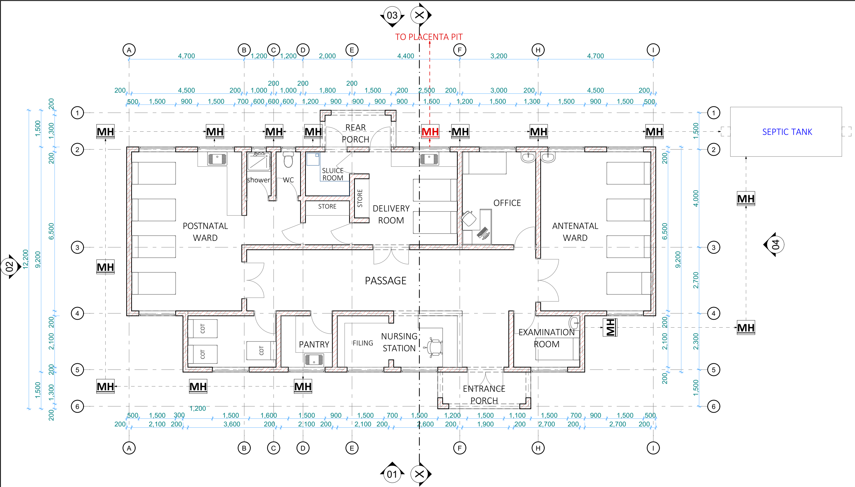
GROUND FLOOR PLAN LAYOUT - SCALE 1:100
