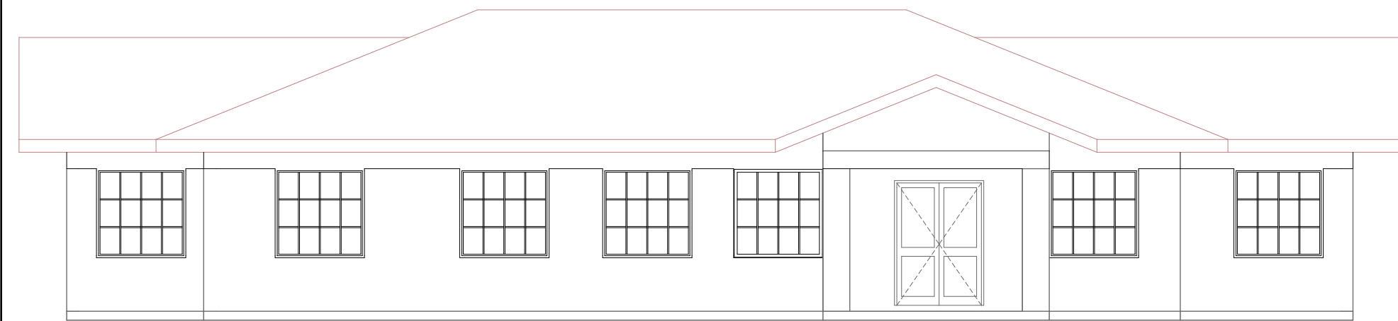
ELEVATION (01) - SCALE 1:100
