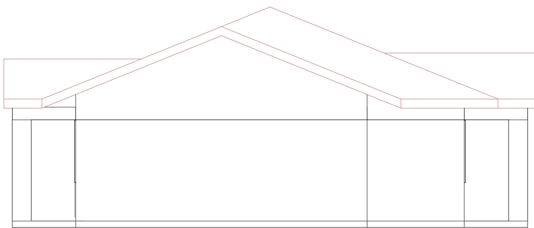
ELEVATION (02) - SCALE 1:100
