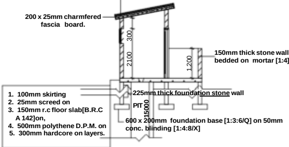
SECTION 01-01
