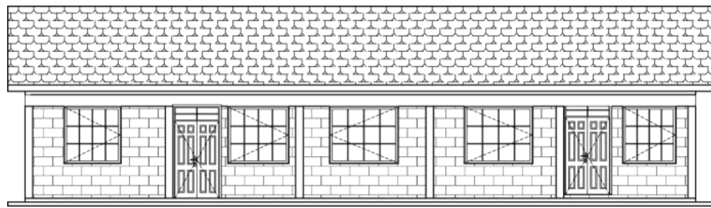
South Elevation
