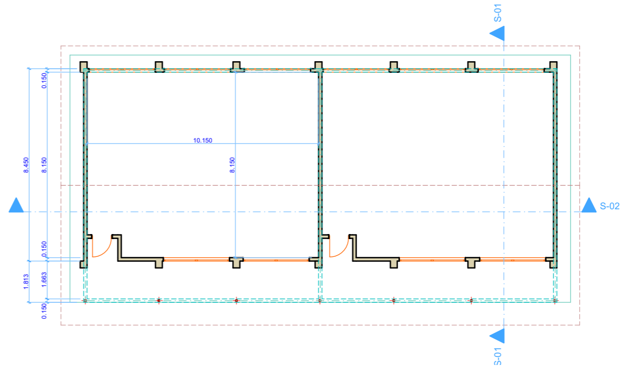
FLOOR PLAN
