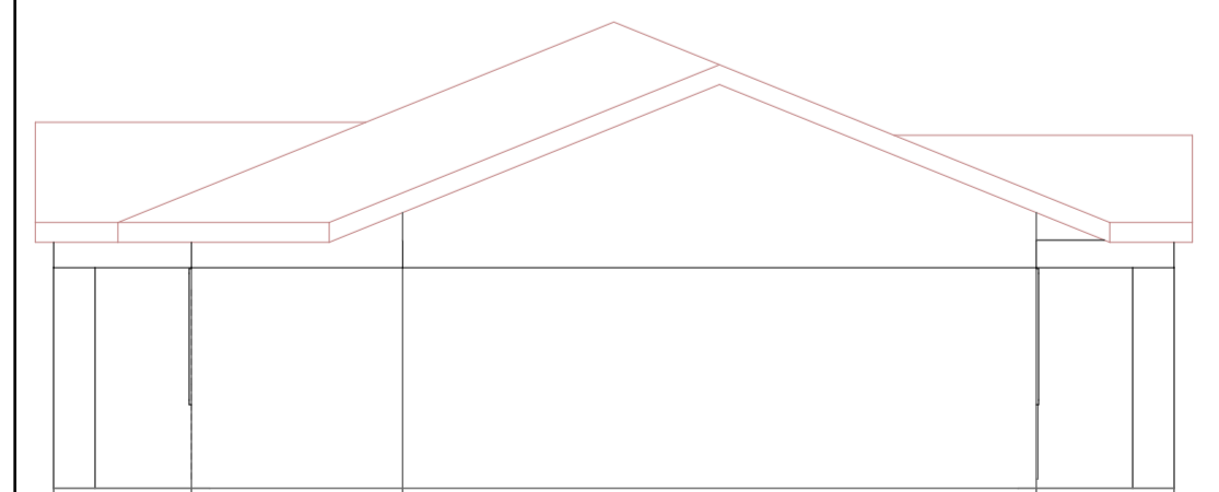
ELEVATION (04) - SCALE 1:100
