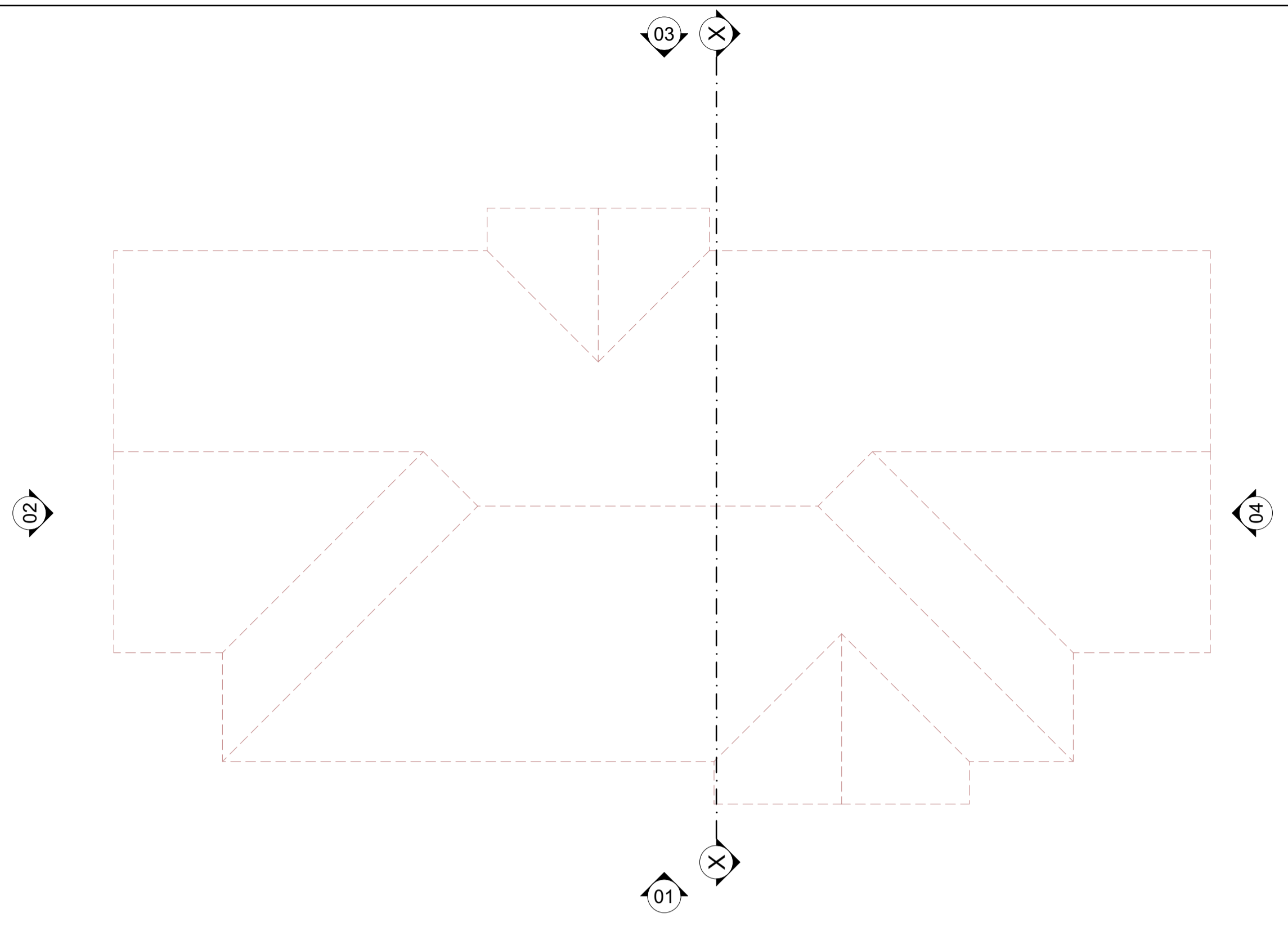
ROOF PLAN LAYOUT - SCALE 1:100
