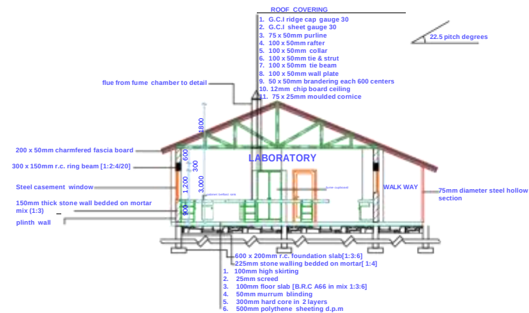
SECTION 01-01
