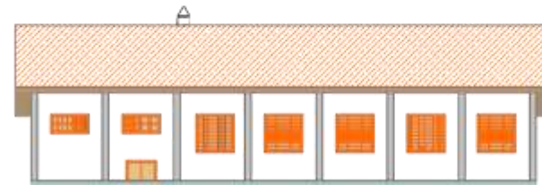
NORTH ELEVATION
