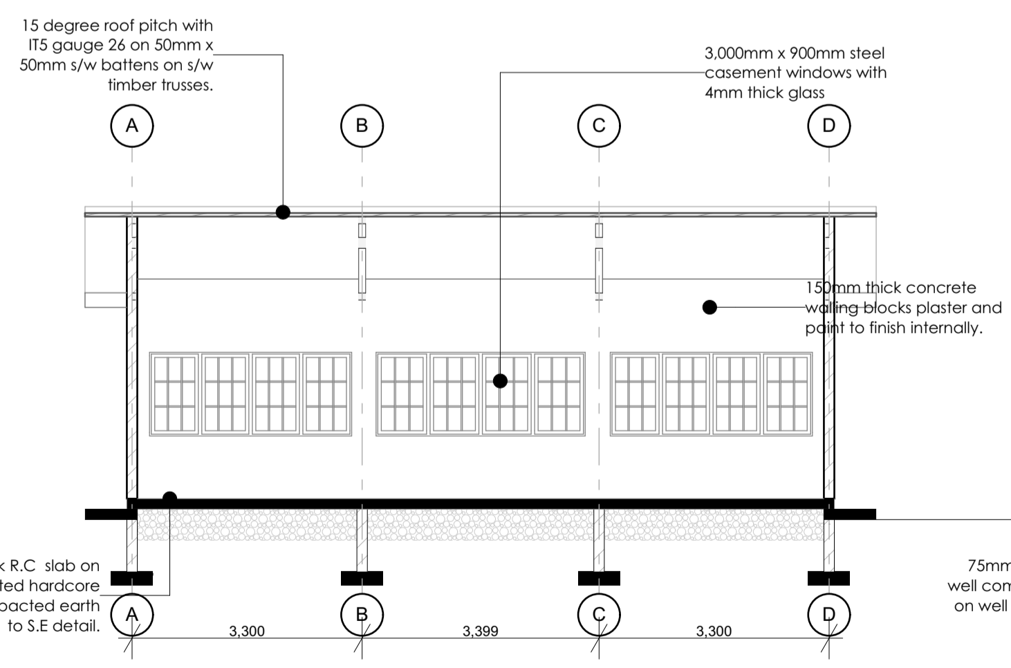
SECTION S-03 1:75
