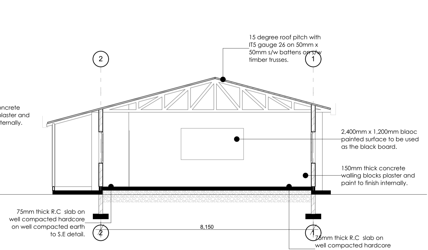
SECTION S-02 1:75
