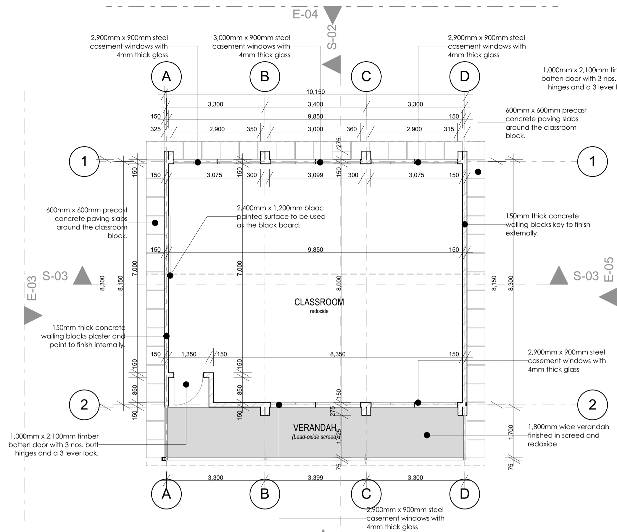
GROUND FLOOR PLAN 1:75
