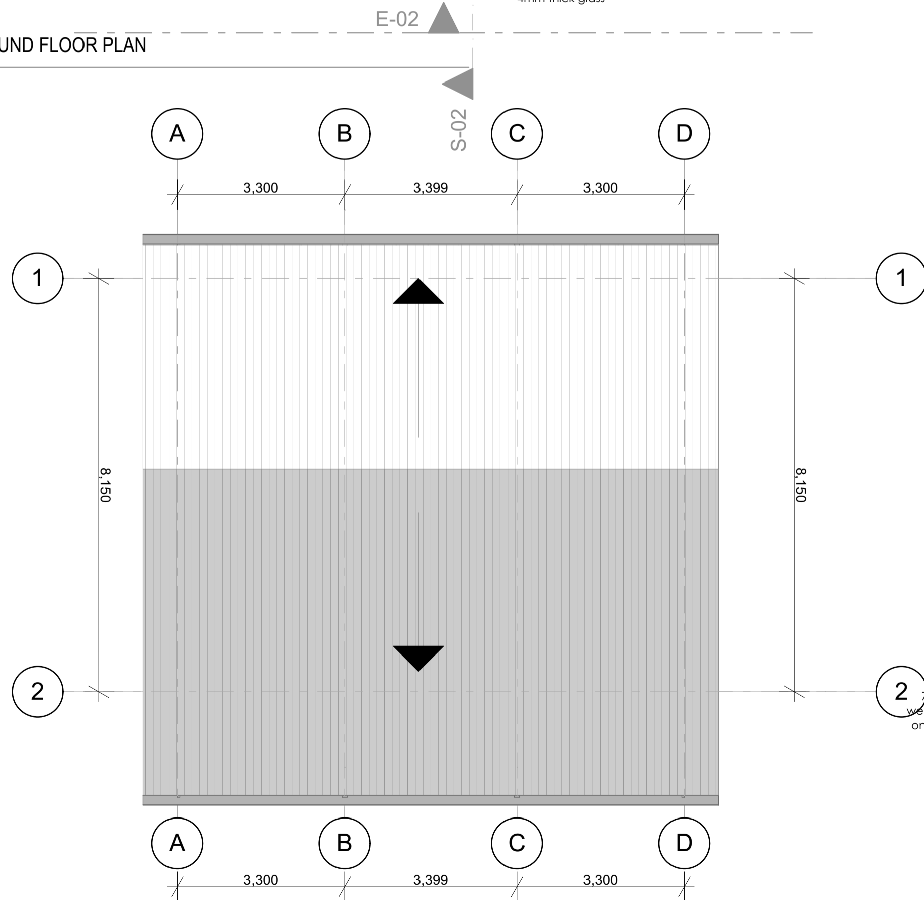
ROOF PLAN 1:75
