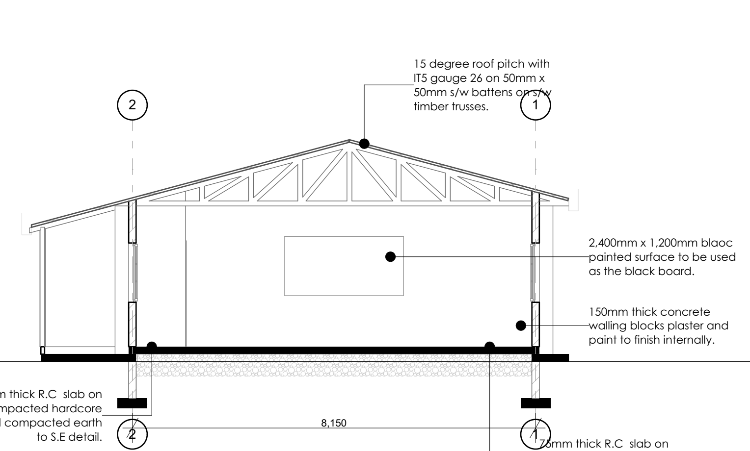
SECTION S-02 1:75
