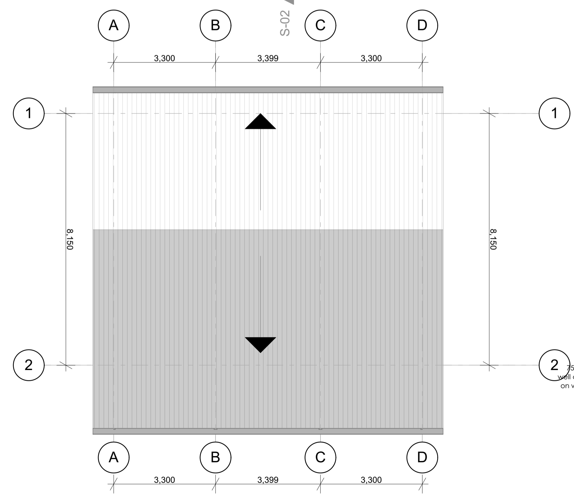
ROOF PLAN 1:75
