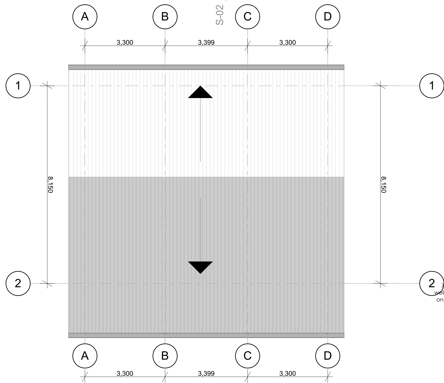
ROOF PLAN 1:75
