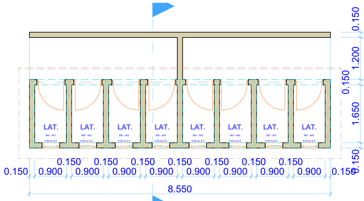
FLOOR PLAN
