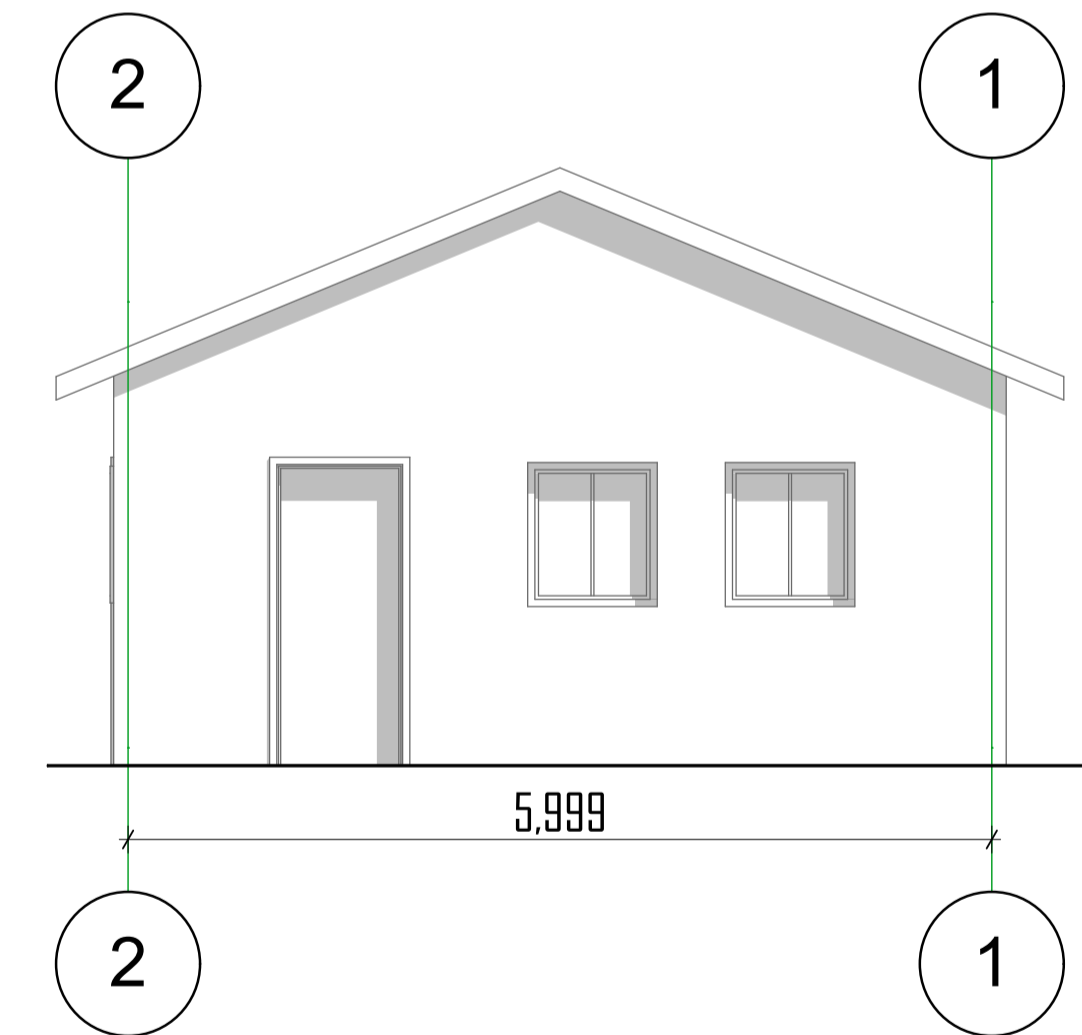
Elevation-04
