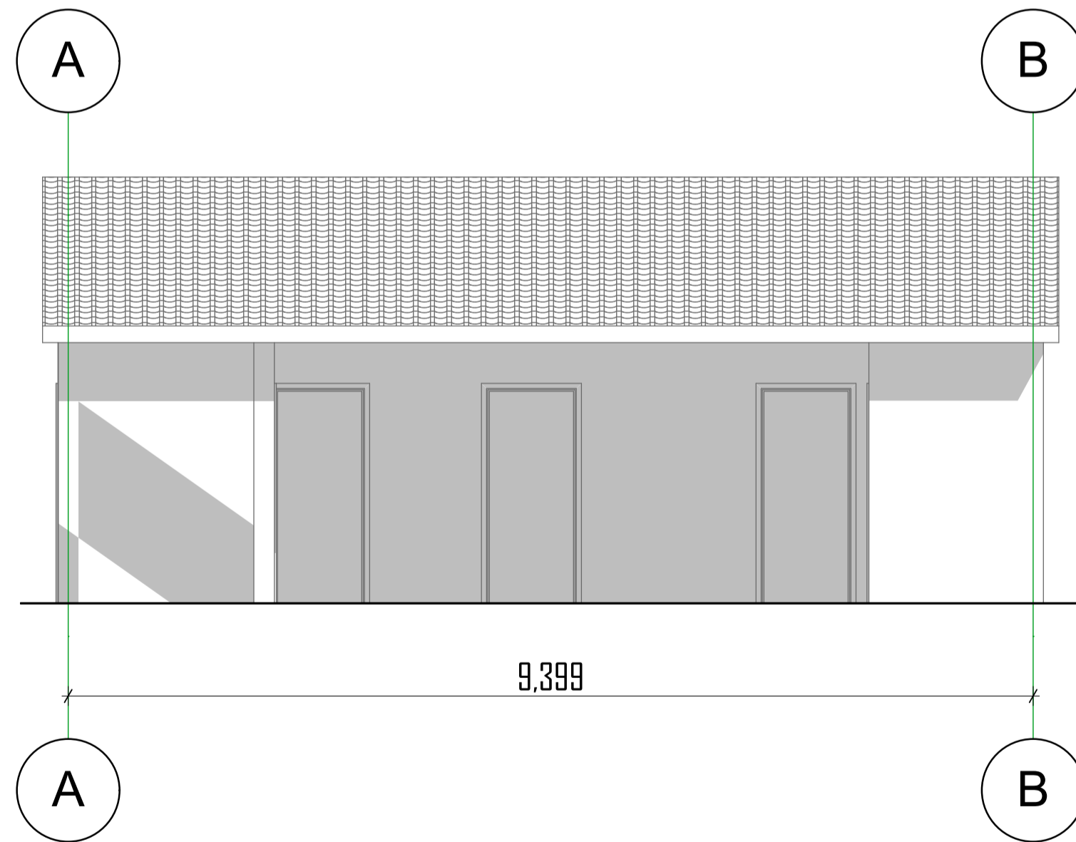
Elevation-03
